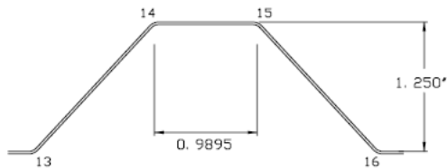
CENTER RIB DETAILS AND INBOARD DETAIL WHEN RUN BEARING LEG
